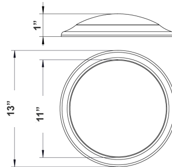
13" x 1" DLS12-MCT-277V
