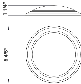
5 4/5" x 1 1/4" DLS6-MCT-277V
